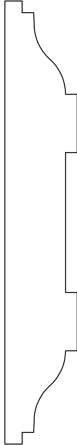
CH-522 2\frac{5}{32} " x 4\frac{3}{4} "
