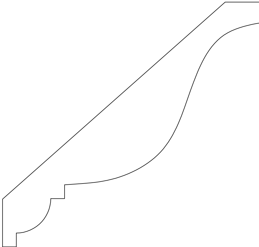
CR-210 4 7 / 16 " x 4 5 / 8 "
